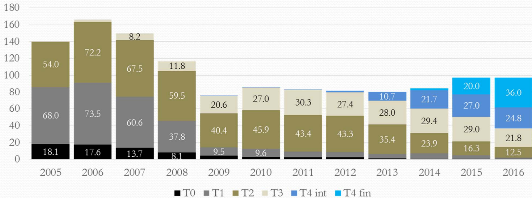
Nonroad Diesel CHE Energy Consumption by Tier, gWh
