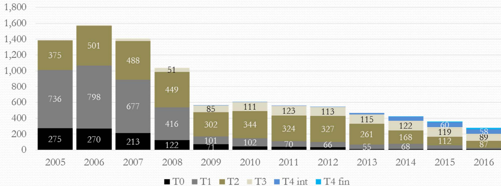
Nonroad Diesel CHE NO x Emissions by Tier, tons
