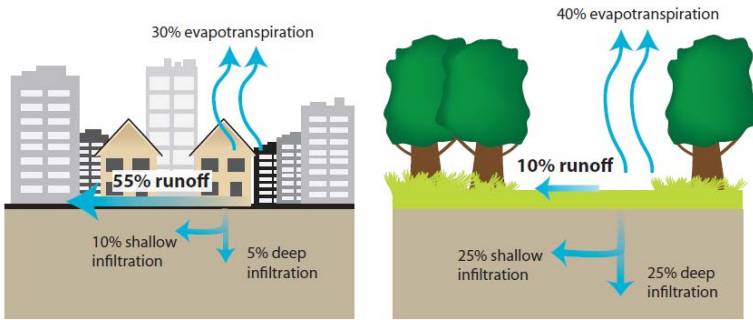
Figure 8: Impervious Surfaces and Reduced Evapotranspiration
