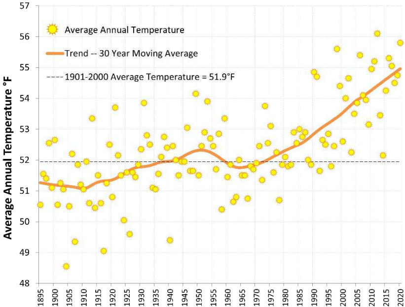
Figure 3: Annual Average Temperature in SE PA and Southern NJ - 1895–2020
