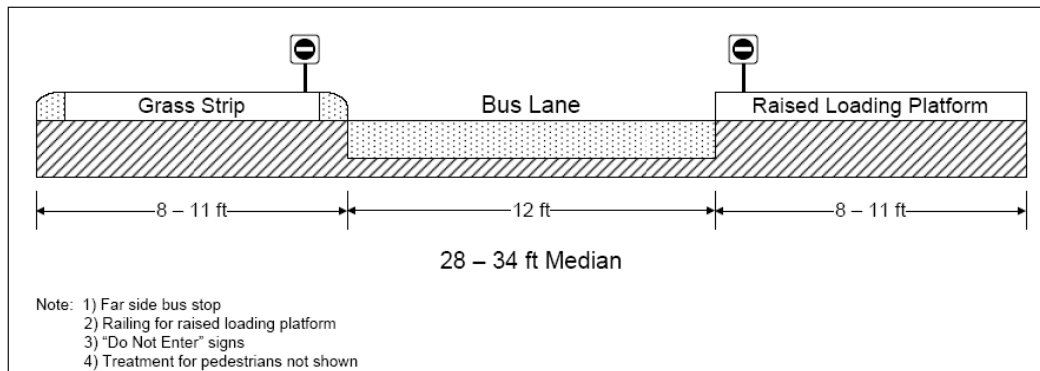
Figure 5: Ideal Busway Configuration at Intersections
