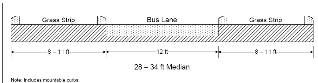
Figure 4: Ideal Mid-block Busway Configuration
