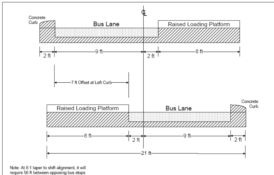
Figure 6: Example of Off-set Alignment at a Bus Stop
